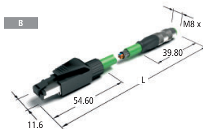
Straight RJ 45/M8 screw type
