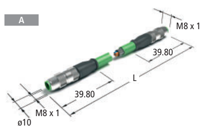
Straight M8 screw type
